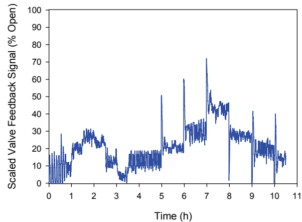
Figure 4-1. Valve position feedback signal
